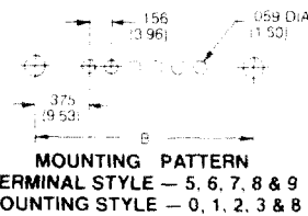
STYLE 3 RIGHT ANGLE, DIP SOLDER TERMINATION STYLE
